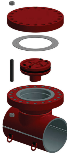
STOPPLE Plus Fitting
